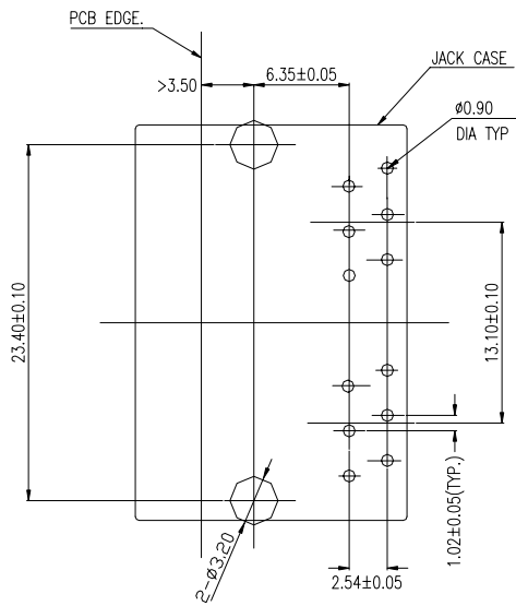
P.C.B. HOLE LAYOUT (Seen from Component Side.)
